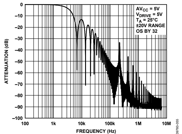
Figure 58. Digital Filter Response for OS \times 32
