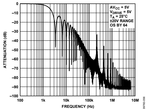
Figure 59. Digital Filter Response for OS \times 64
