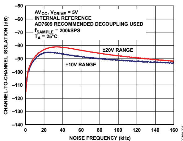
Figure 25. Channel-to-Channel Isolation
