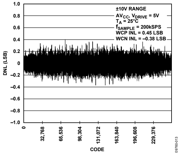
Figure 14. Typical DNL, \pm 10V Range
