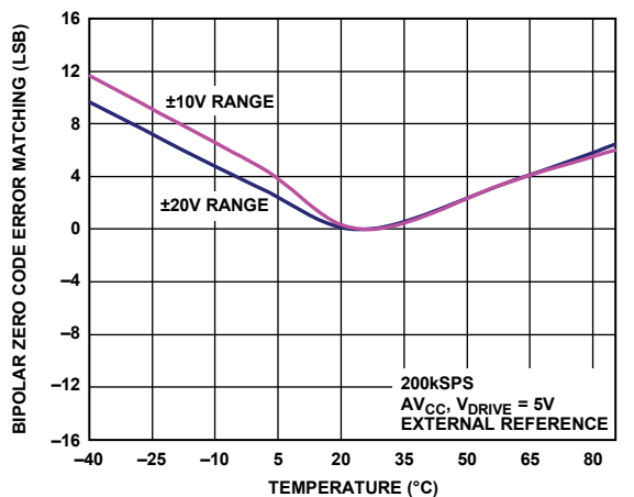
Figure 24. Bipolar Zero Code Error Matching Between Channels
