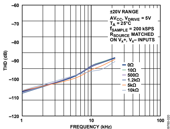
Figure 21. THD vs. Input Frequency for Various Source Impedances, \pm 20 V Range
