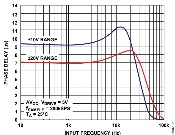
Figure 36. Analog Antialiasing Filter Phase Response
