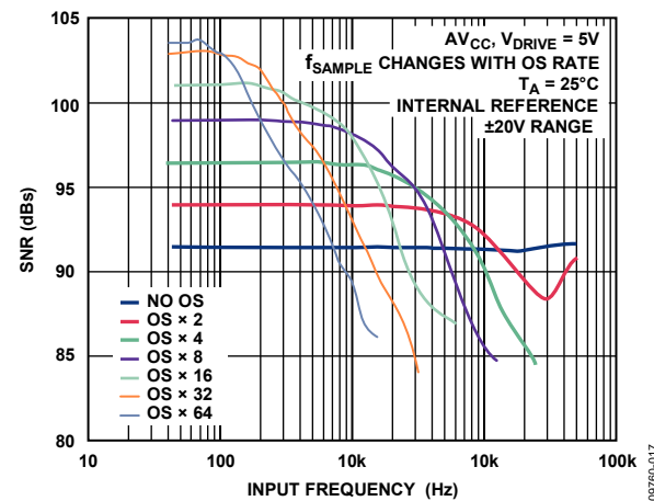
Figure 19. SNR vs. Input Frequency, \pm 20V Range
